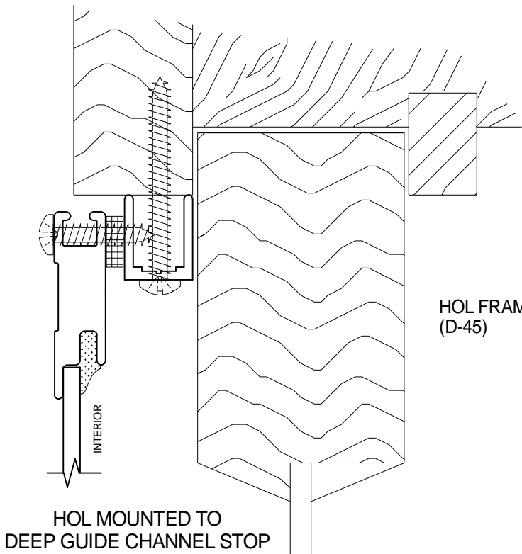
1 HEAD DETAIL SCALE: FULL JAMB SIMILAR
